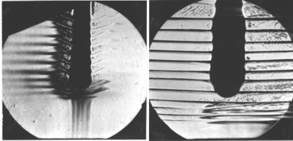
Freezing ice on a cylindrical refrigerator in a continuously stratified water solution of sodium chloride
